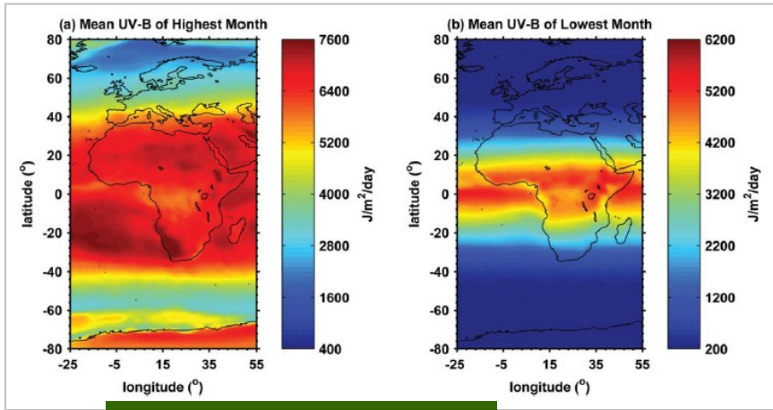
UV incidence across Africa. Uganda is situated at latitude 0.
